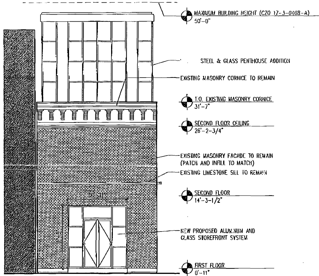
1 PROPOSED SOUTH FACADE 1/8" = 1'-0"
