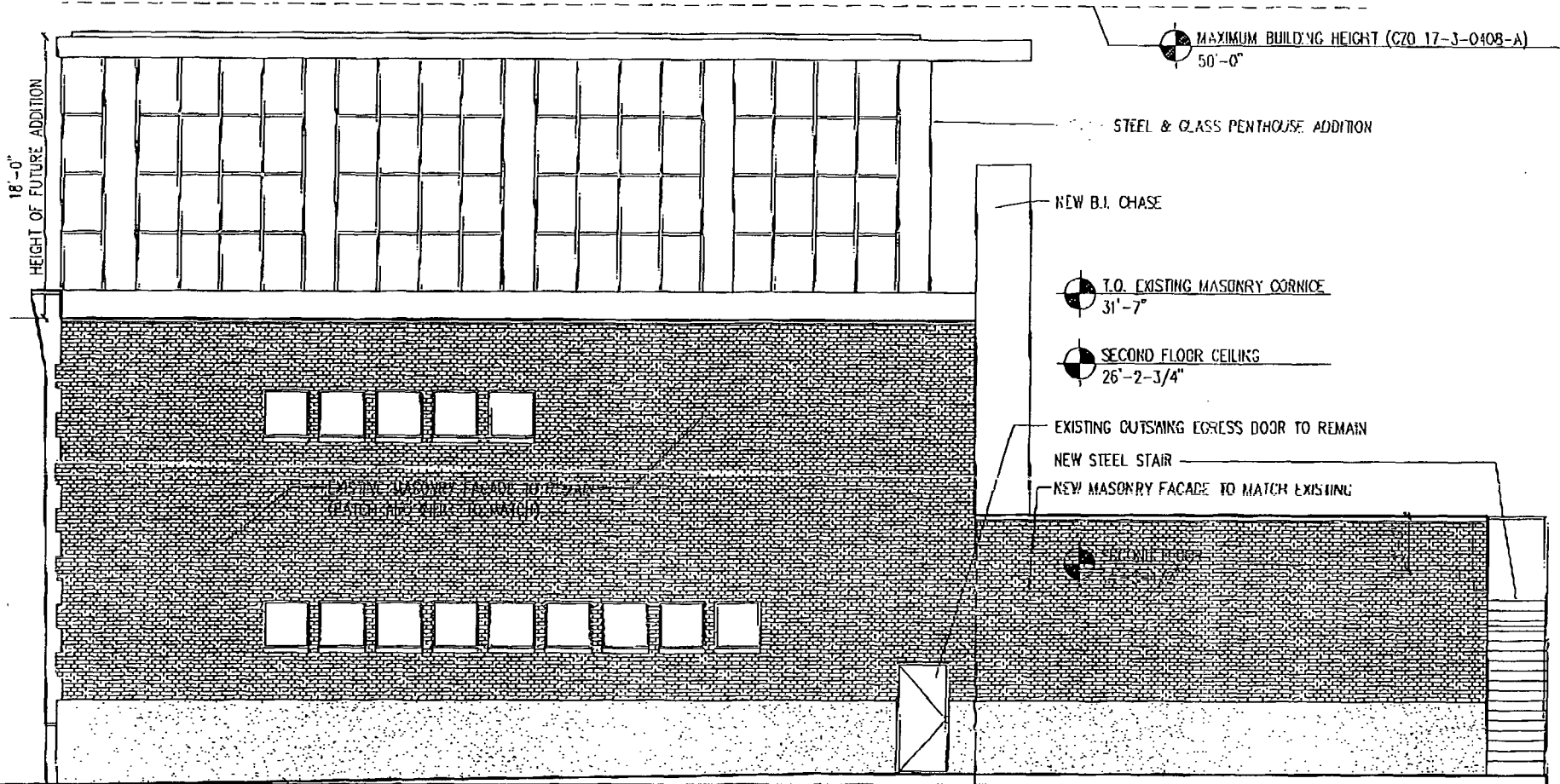
2 PROPOSED EAST FACADE 1/8" = 1'-0"
