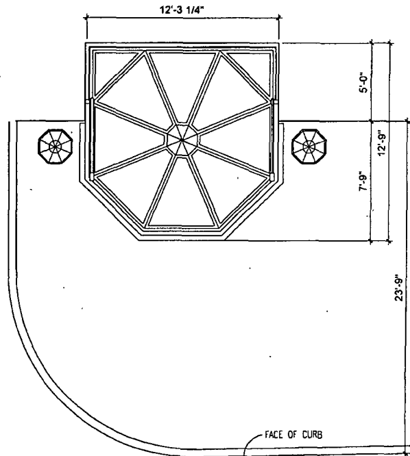
ENLARGED PLAN
