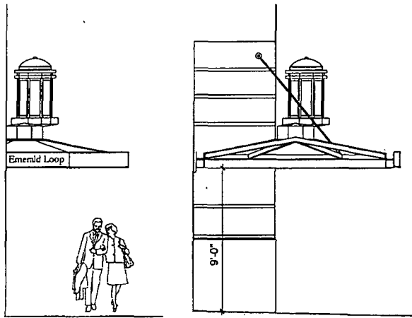
ELEVATION SECTION
