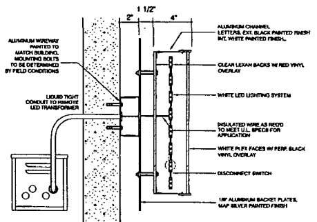
SECTION THRU INTERNALLY ILLUM. CHANNEL LTR.
