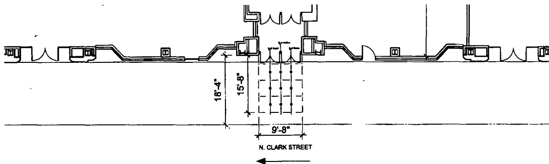
2 PLAN 1/16" = 1'-0"
