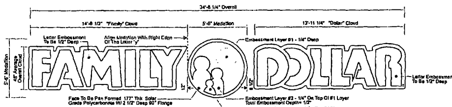
Front View - 48" Linear Cloud / 5'-6" Medallion Scale: 1/4" = 1'-0"
