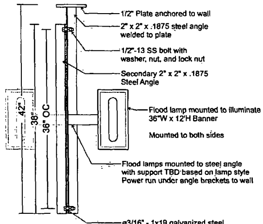
Top Section View Power Provided at 277V
