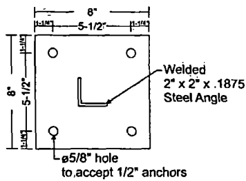
Mounting Plate
