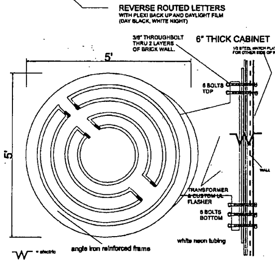
DOUBLE-SIDED WALL MOUNTED (UL APPROVED) ROUTED REVERSE CABINET WITH NEON CENTER
