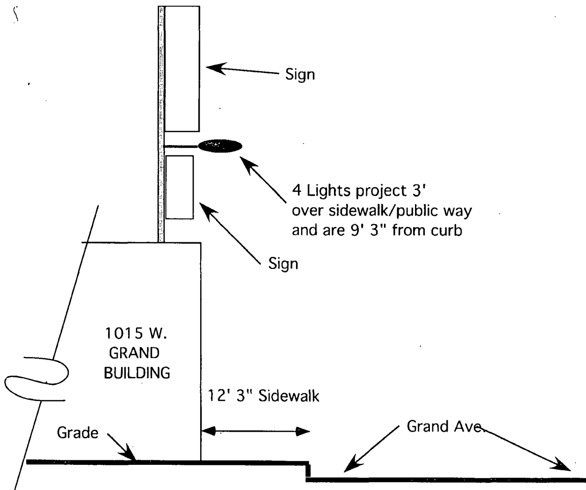
Partial Side Elevation
