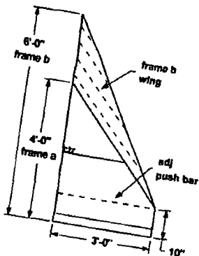
ISOMETRIC VIEW W101
