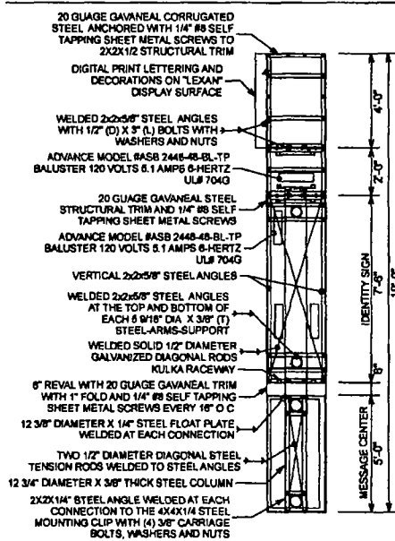
BOX CABINET DETAIL (4) A-1 NOT TO SCALE
