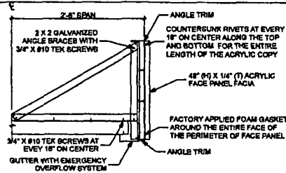
LOGO SECTION (5) A-1 NOT TO SCALE
