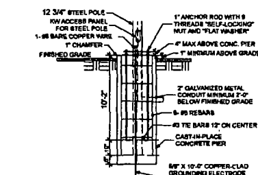
CONCRETE FOOTING (2) A-1 NOT TO SCALE
