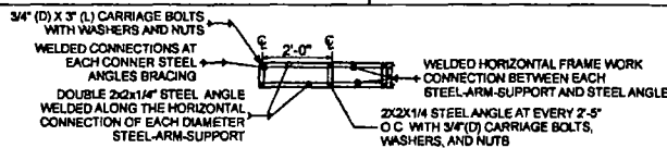
STEEL-ARM-SUPPORT (3) A-1 NOT TO SCALE
