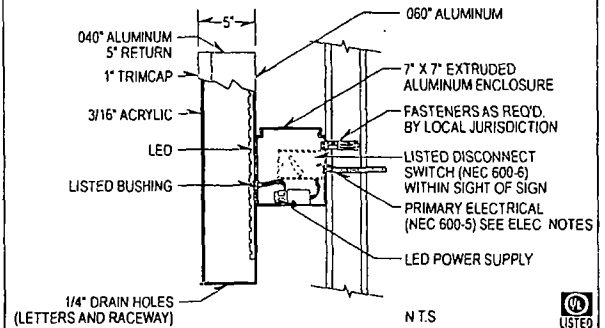
CHANNEL LETTER - TYPICAL SECTION - FRONT-LIT PLASTIC FACE
