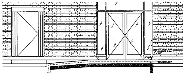
1 EXISTING RAMP SECTION SCALE 1" = 10'
