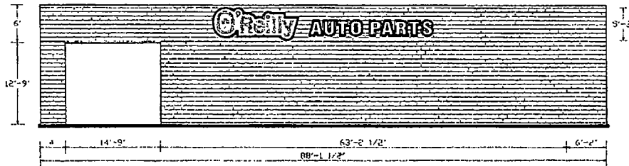
EAST ELEVATION FACING MILWAUKEE AVE
