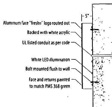
FRESHII LOGO ROUTED CABINET
