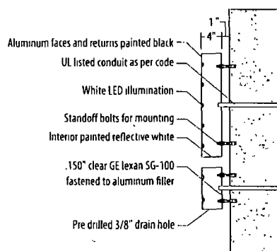
EAT. ENERGIZE. CHANNEL LETTERS
