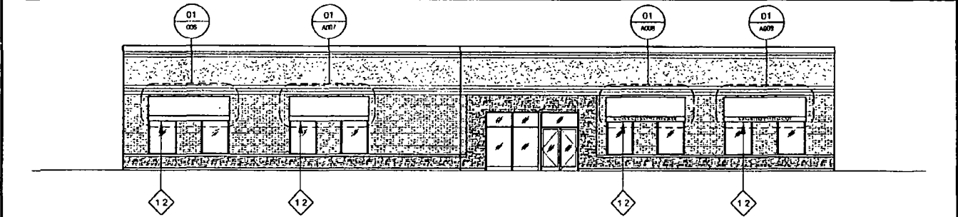
02 WEST ELEVATION - MARSHFIELD AVENUE SCALE N.T.S.
