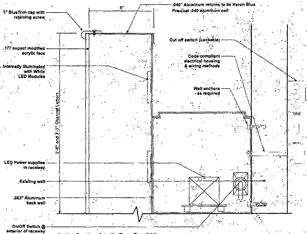
Letter Section Acrylic Face Detail View -
