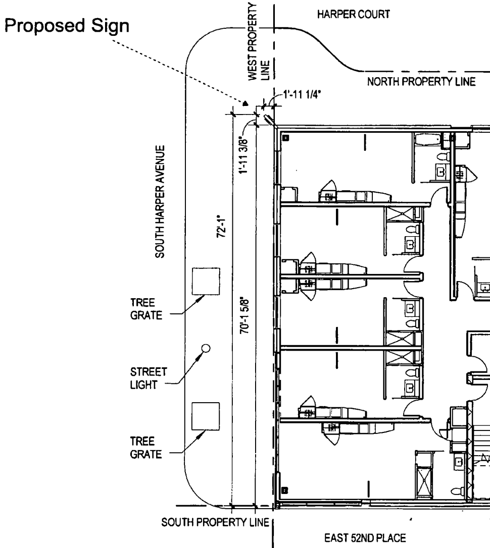
Hyatt Place at Harper Court Plan View (at Third Floor)
