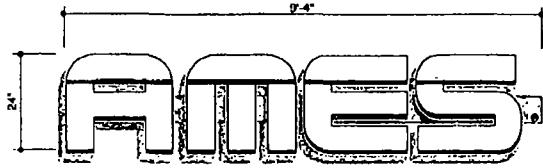
INDIVIDUAL INT. NEON ILLUMINATED LETTER DISPLAY 1/2" = 1'-0"
