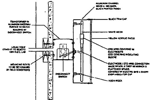
RACEWAY MOUNT INTERNALLY ILLUM. CHANNEL LTR.
