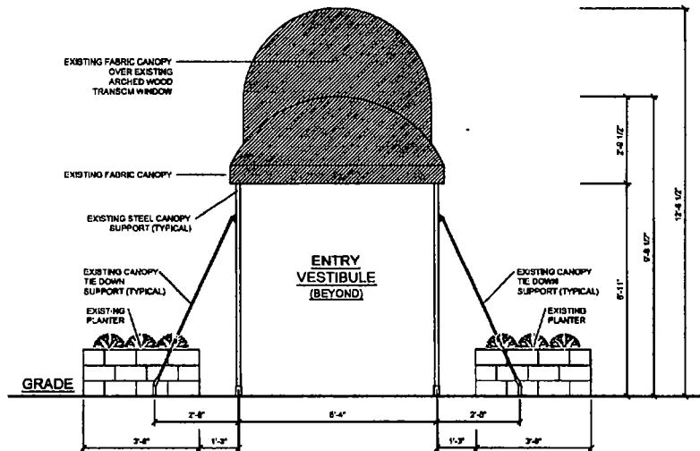
5000 S. EAST END BLDG. CHICAGO, IL 1 EXISTING CANOPY ELEVATION NORTH AT NORTH ENTRANCE SCALE : 1/4" = 1'-0"
