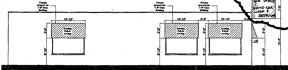
South Elevation
