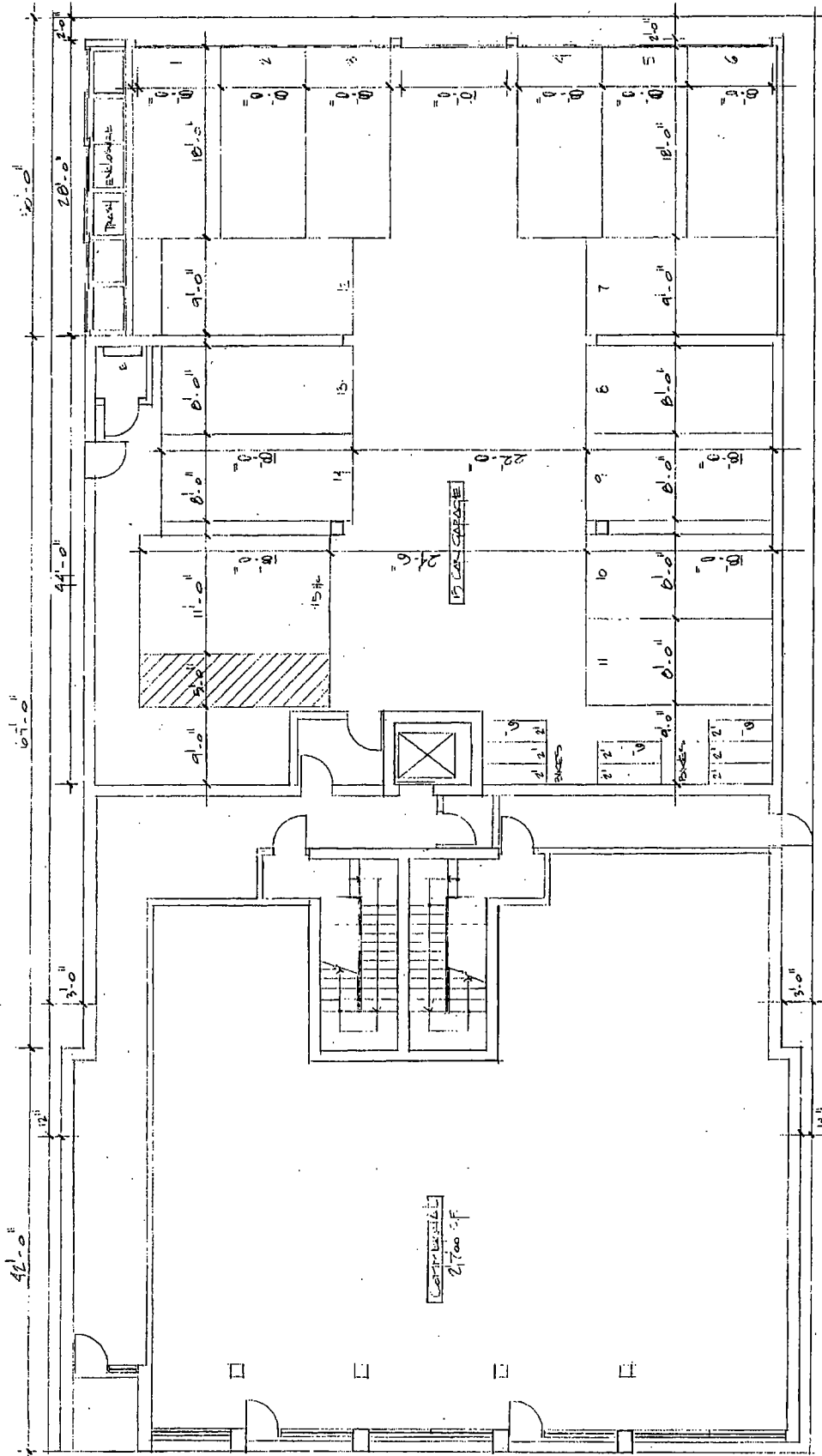
1st Floor Plan 1/8" = 1'-0"
