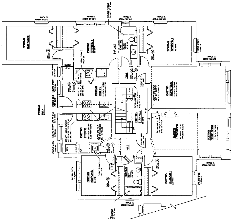
SECOND FLOOR PLAN - NORTH UNIT
