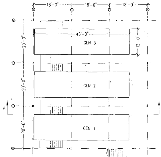
STACKED GENERATOR ENCLOSURE SCHEME - LOWER LEVEL
