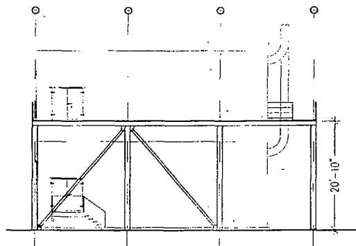
STACKED GENERATOR ENCLOSURE SCHEME - SECTION A-A
