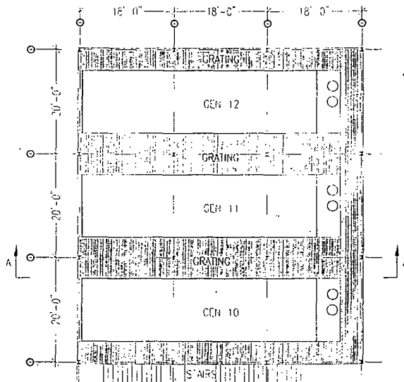
STACKED GENERATOR ENCLOSURE SCHEME - UPPER LEVEL
