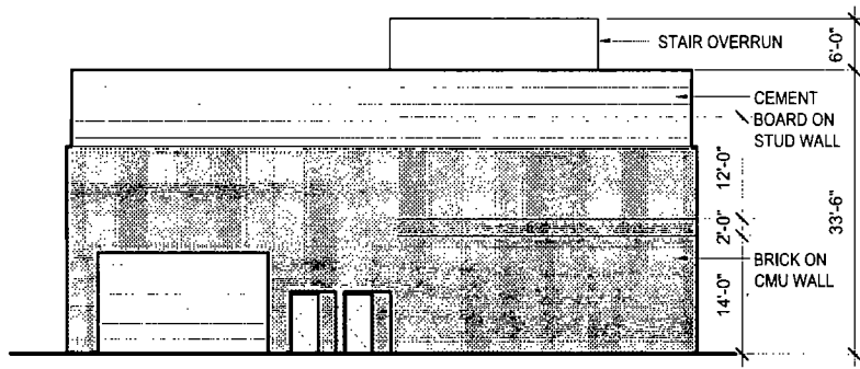
4 SOUTH ELEVATION SCALE: 1/16" = 1'-0"
