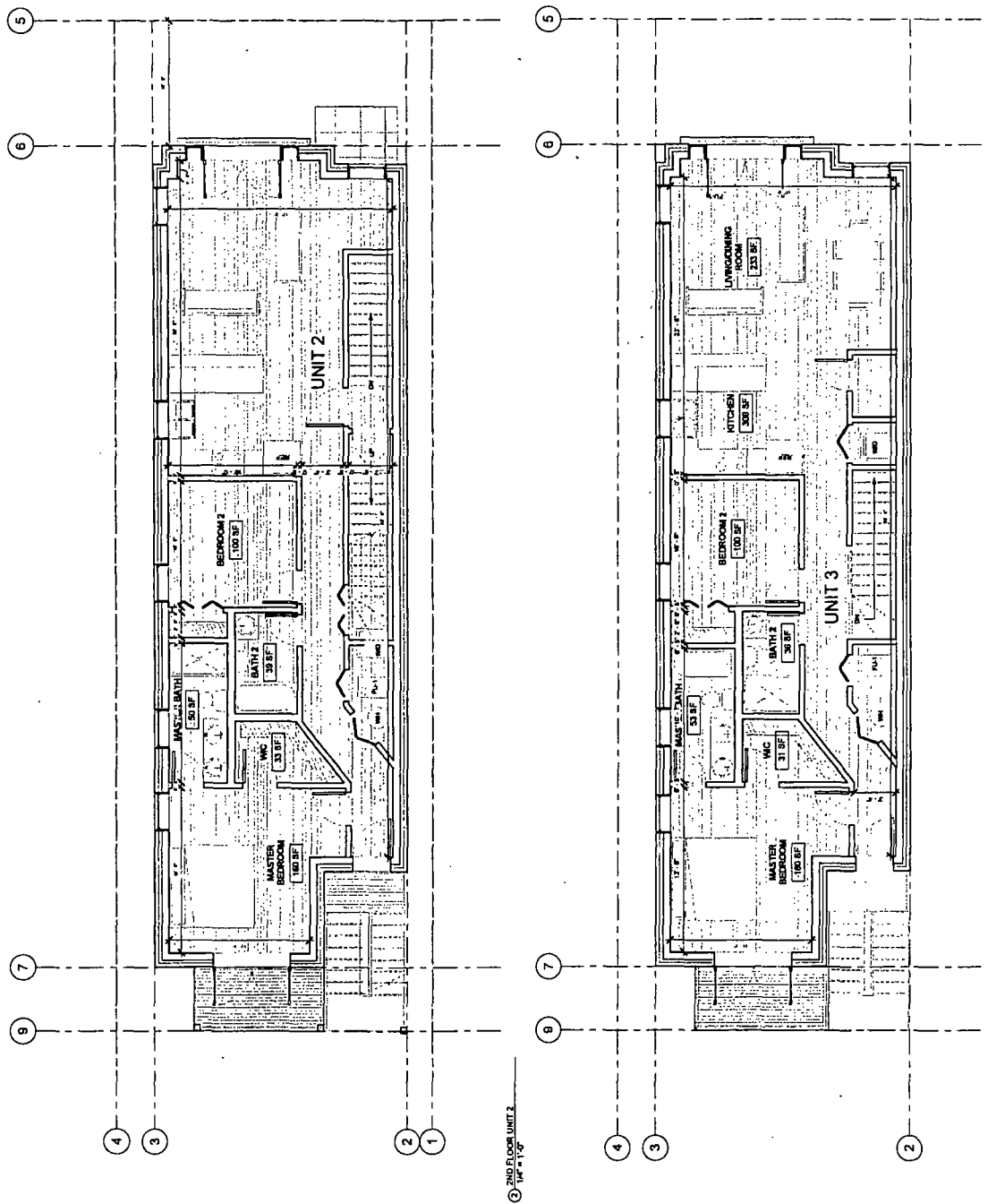
① 3RD FLOOR UNIT 3 1/4" = 1'-0"
