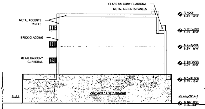
1 Northwest Elevation SCALE: 1/4"=1'-0"
