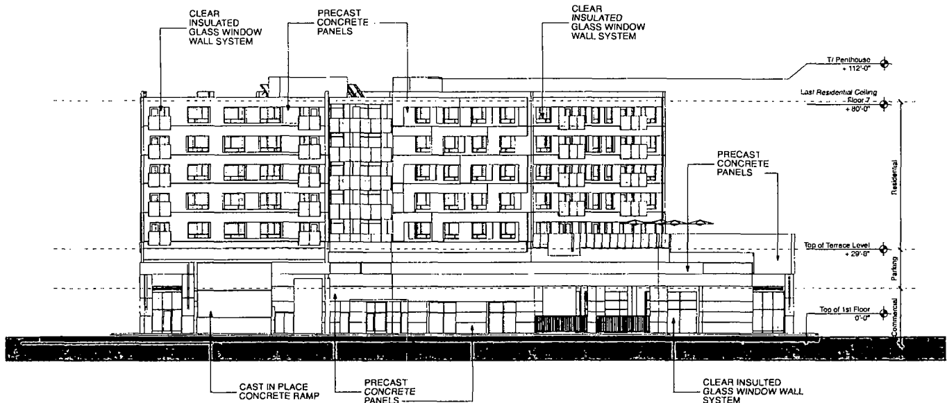
North Elevation
