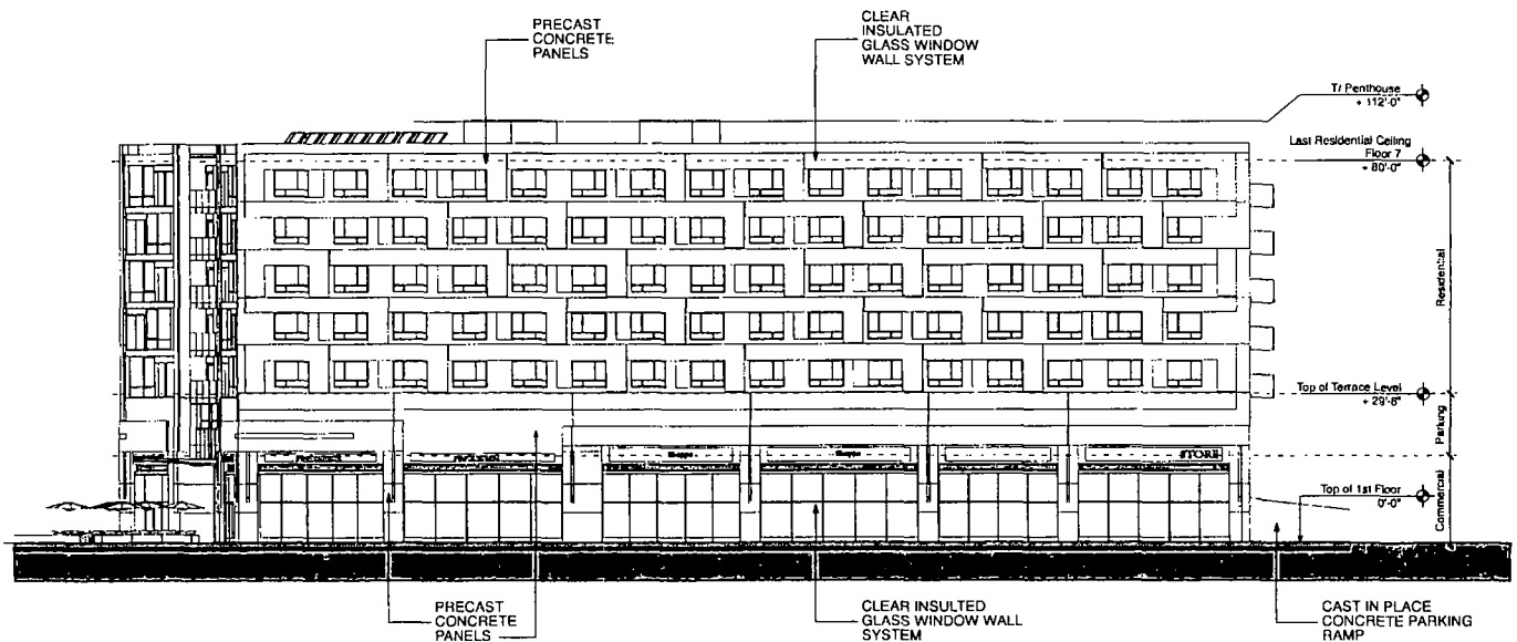
East Elevation
