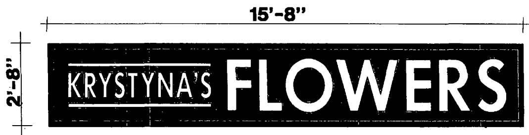
2'-8"x15'-8" SINGLE FACE SIGN
