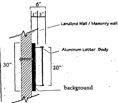
CROSS SECTION DETAIL
