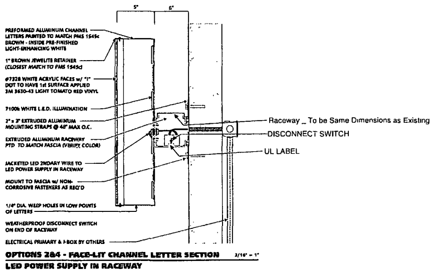
Typical Detail - Led Channel Letters on Raceway
