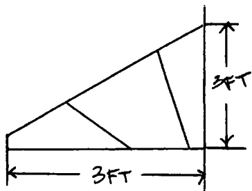
AWNING 1, 2, 3 PROFILE VIEW
