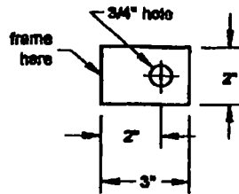
SIDE MOUNTING TABS (4)
