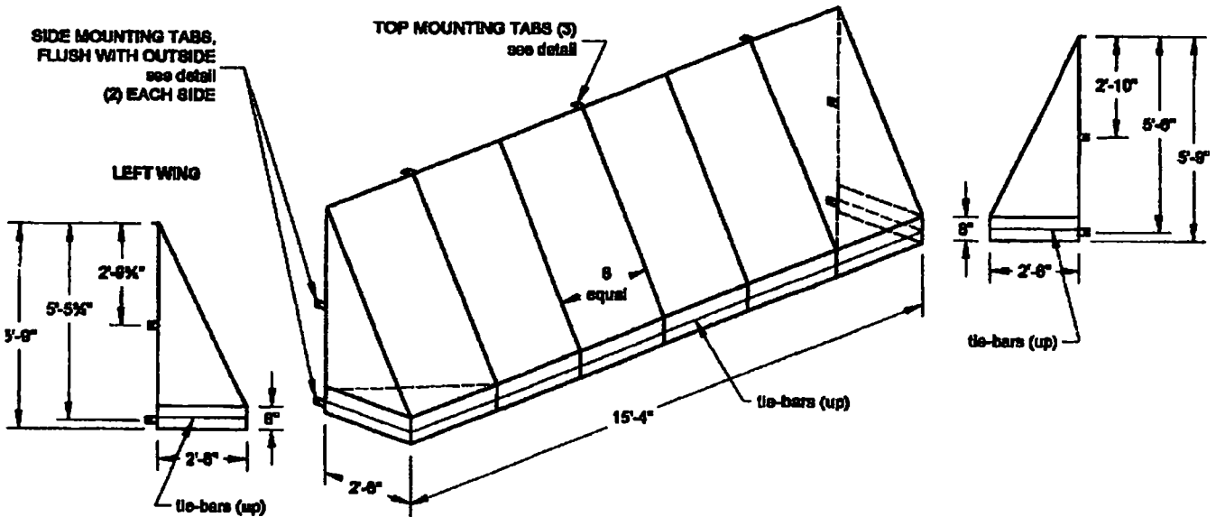
ISOMETRIC VIEW
