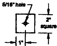
TOP MOUNTING TABS (3)
