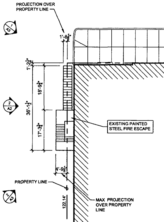
1 FIRE ESCAPE PLAN
