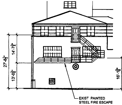
2 FIRE ESCAPE ELEVATION
