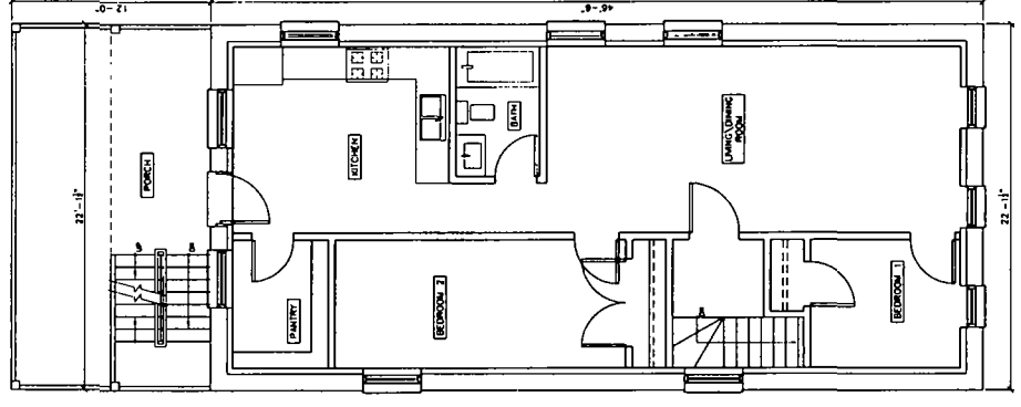
EXIST. SECOND FLOOR PLAN SCALE 1/4" = 1'-0"
