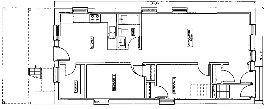
EXIST. FIRST FLOOR PLAN SCALE 1/4" = 1'-0"
