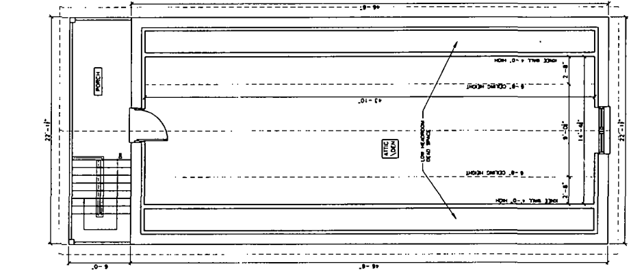
EXIST. ATTIC FLOOR PLAN SCALE 1/4" = 1'-0"
