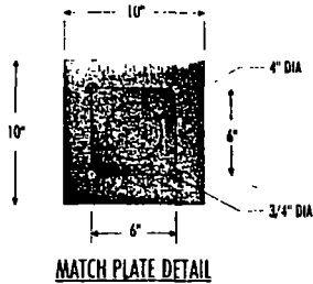
MATCH PLATE DETAIL
