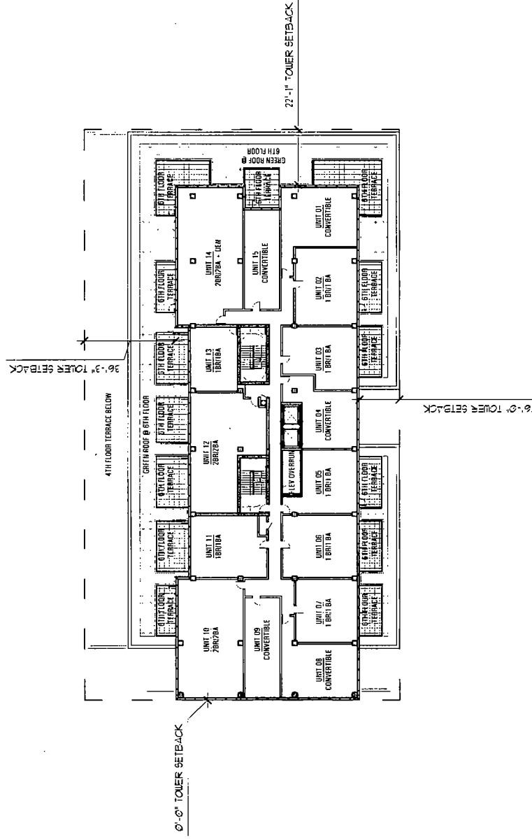
① SIXTH FLOOR PLAN SCALE 1/32" = 1'-0"
