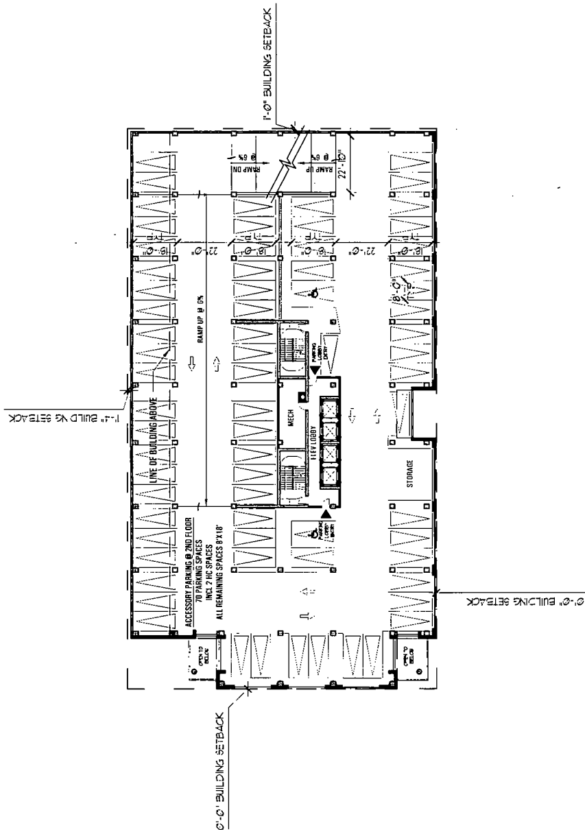
① SECOND FLOOR PLAN SCALE: 1/32" = 1'-0"
