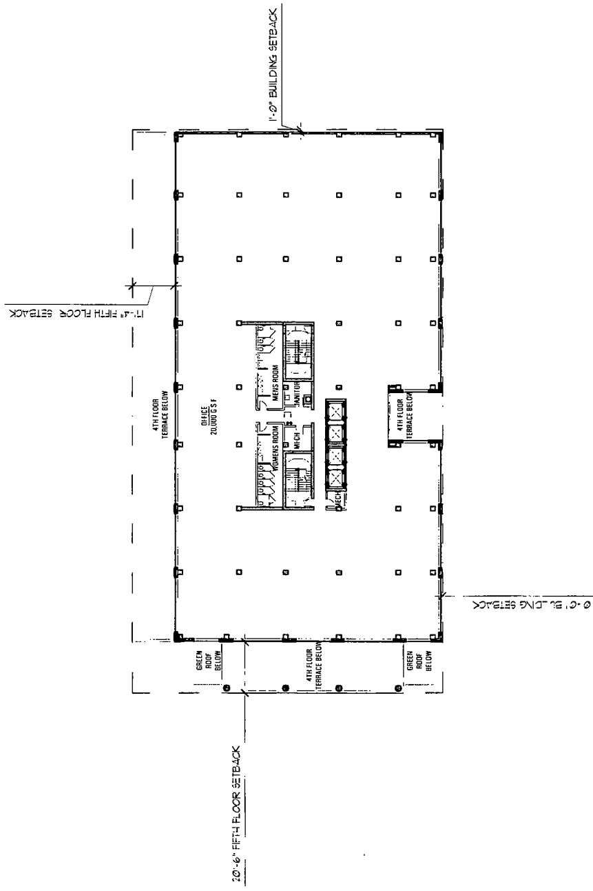
① FIFTH FLOOR PLAN SCALE: 1/32" = 1'-0"
