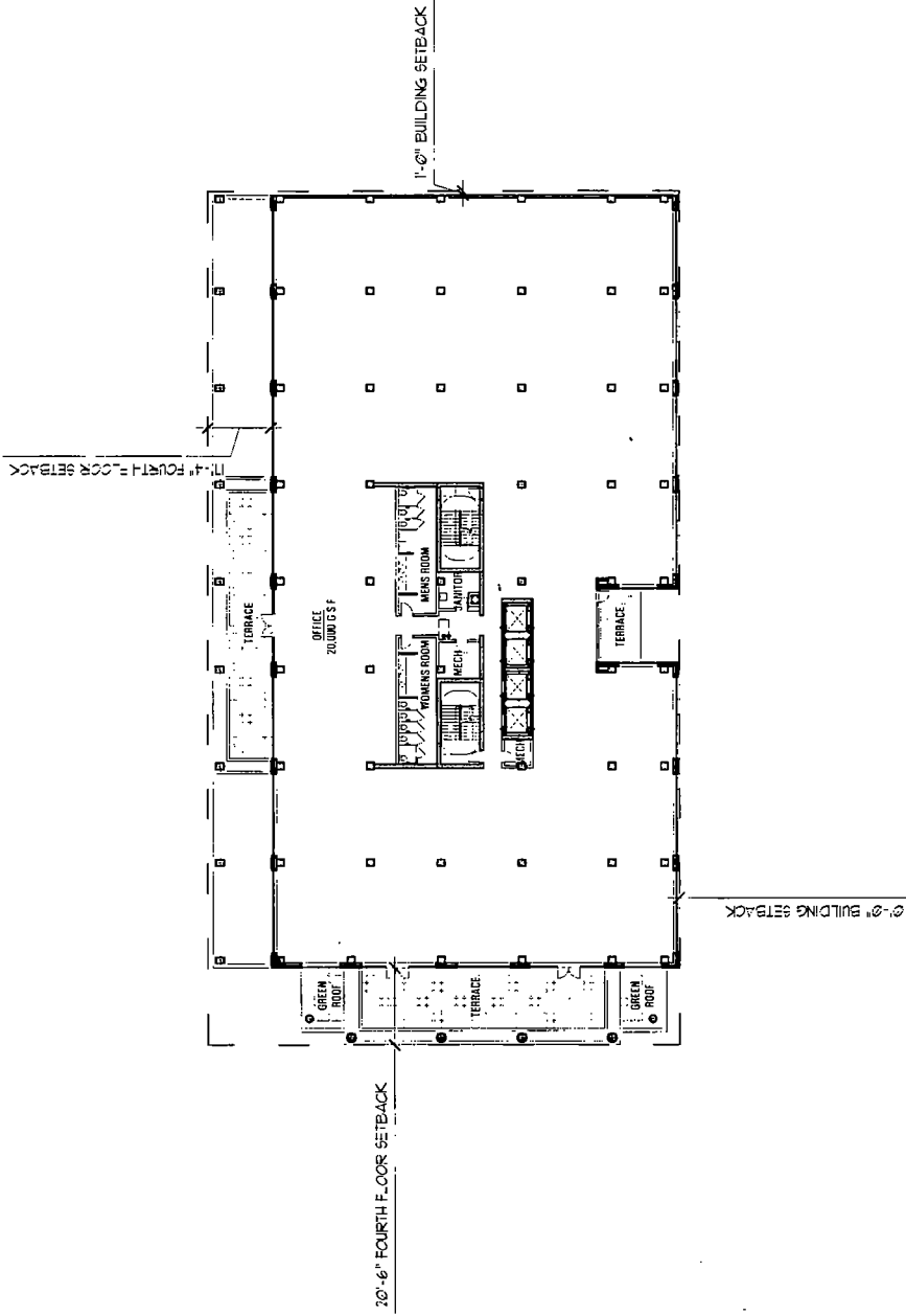
① FOURTH FLOOR PLAN SCALE 1/32" = 1'-0"
