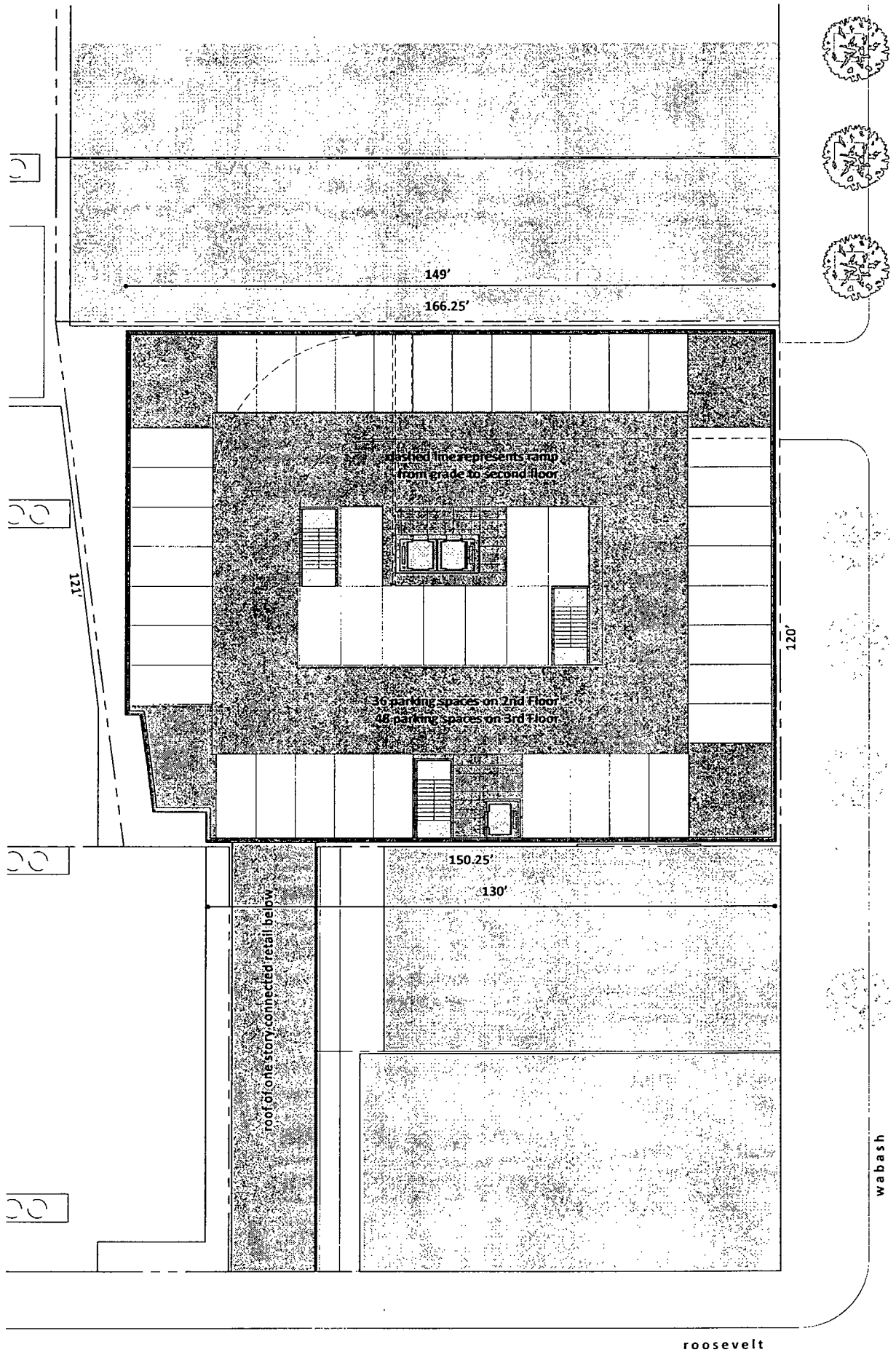
Parking Floor Plan @ 3 (2 is similar)
