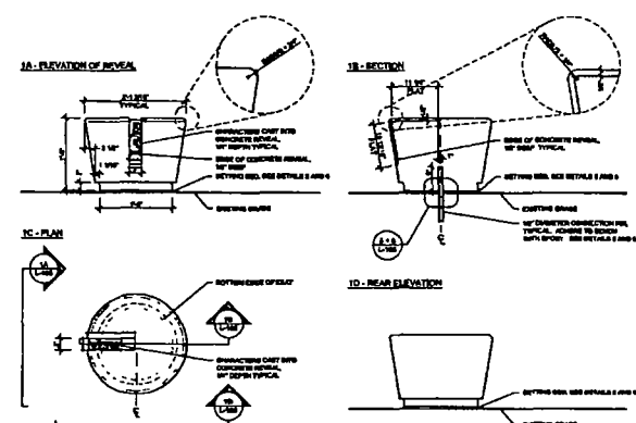
1 PRECAST CONCRETE BLOCK TYPE 'A' - SMALL 1" = 1'-0"
