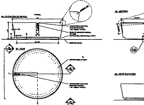
4 PRECAST CONCRETE BLOCK TYPE 'B' - LARGE 1" = 1'-0"
