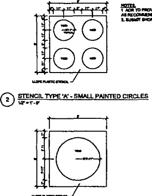
2 STENCIL TYPE 'A' - SMALL PAINTED CIRCLES 1/2" = 1'-0"
