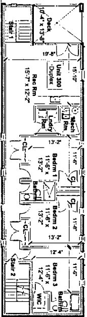
5 FOURTH FLOOR PLAN P2 Scale: 1/8\"/>
