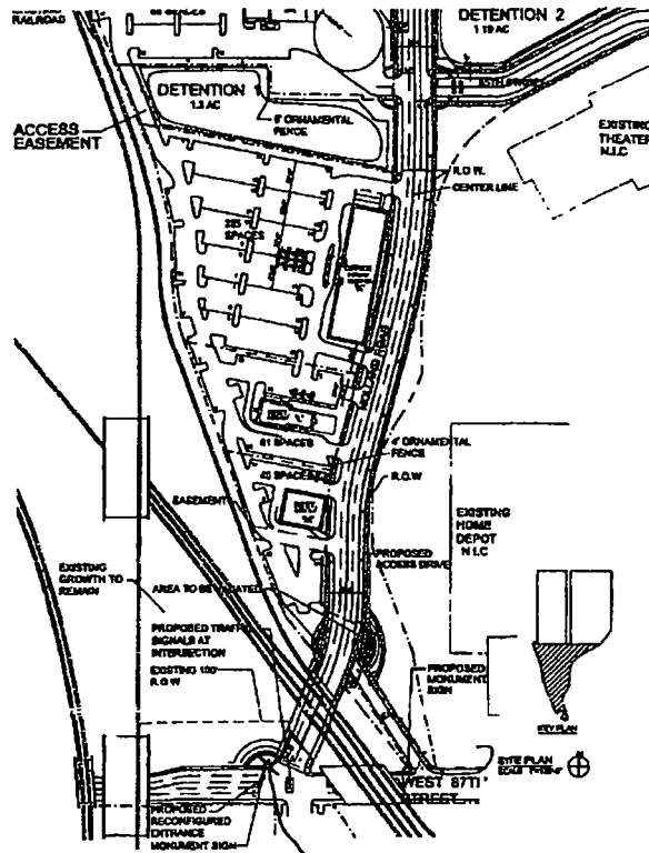
Site Plan. (Page 3 of 3)
