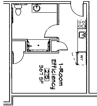
Typical 1-Room Efficiency Unit 10'0" x 11'0"
