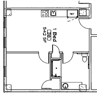
Typical 1-Bedroom Unit 1/8" = 1'-0"
