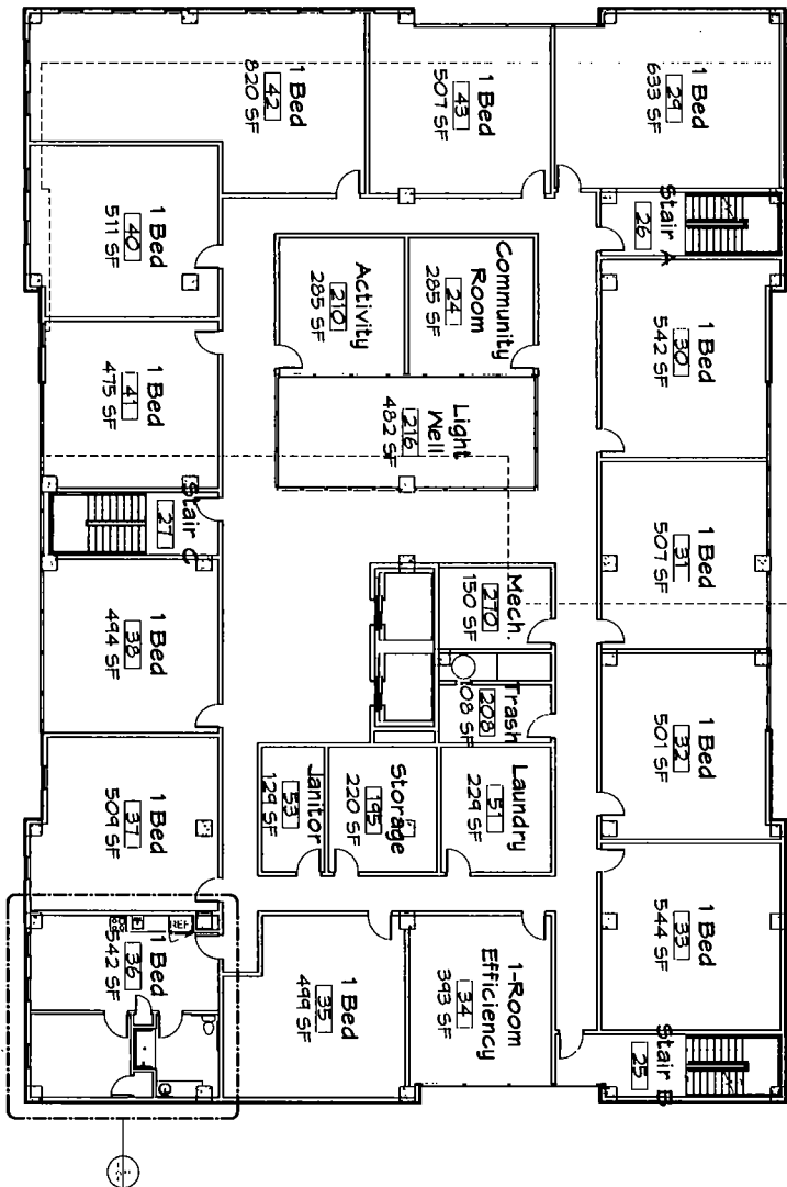
Typical Third Floor - 7th Floor 1/8" = 1'-0"
