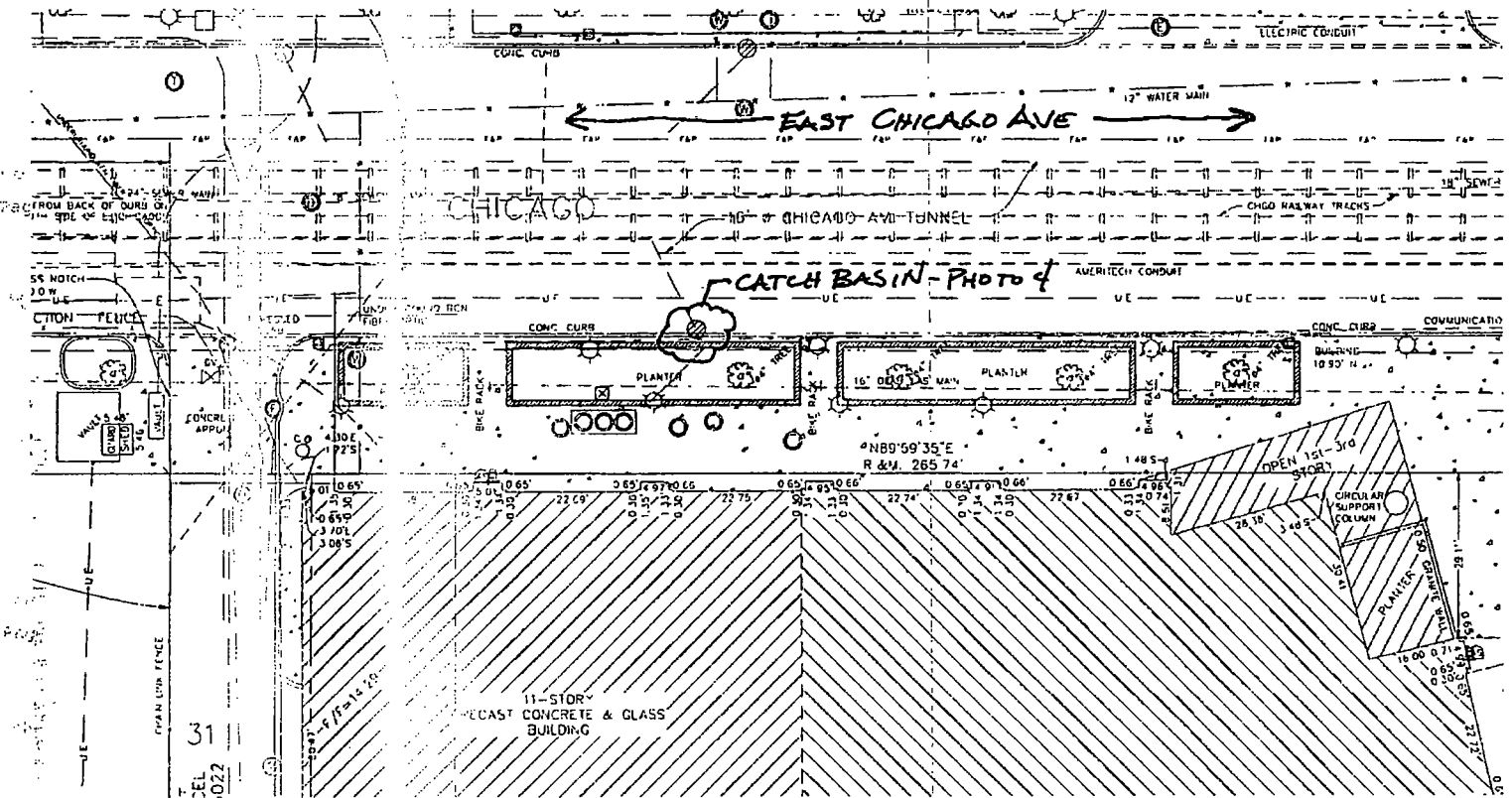
PARTIAL SITE PLAN CATCH BASIN E. CHICAGO AVE
