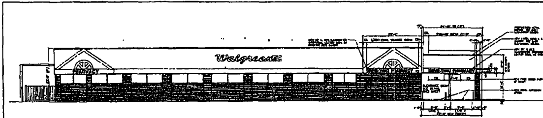
PARTIAL SOUTH ELEVATION - REVISED NEW WOOD
