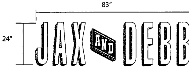
INDIVIDUAL INT. LED ILLUMINATED LETTER DISPLAY
