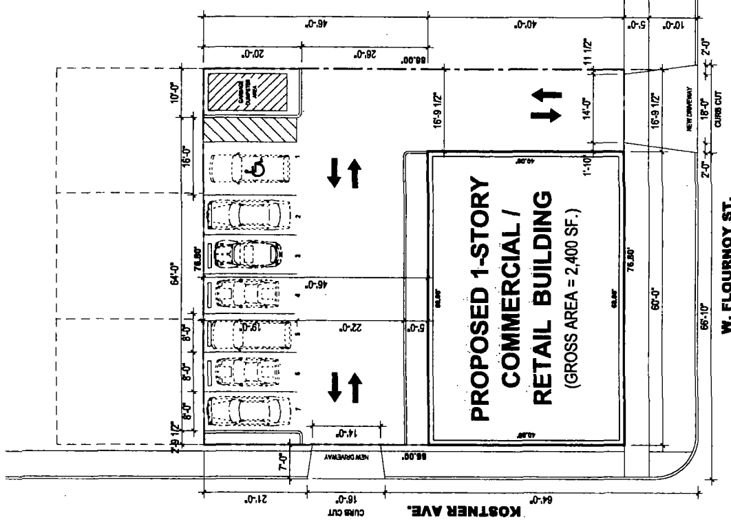
1 SITE PLAN
