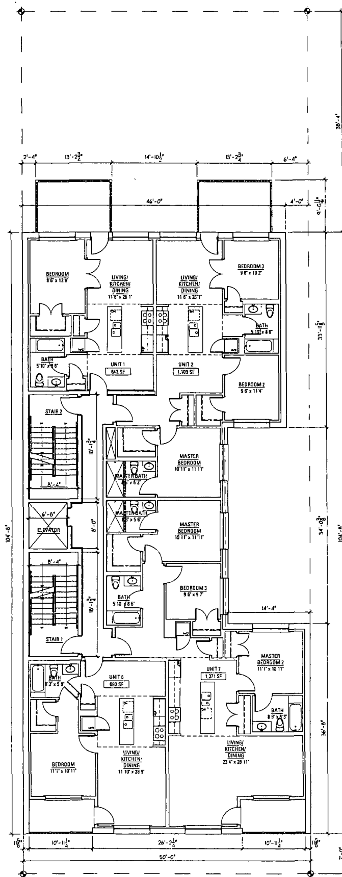
5TH - 7TH FLOOR PLAN - 4,479 SF
