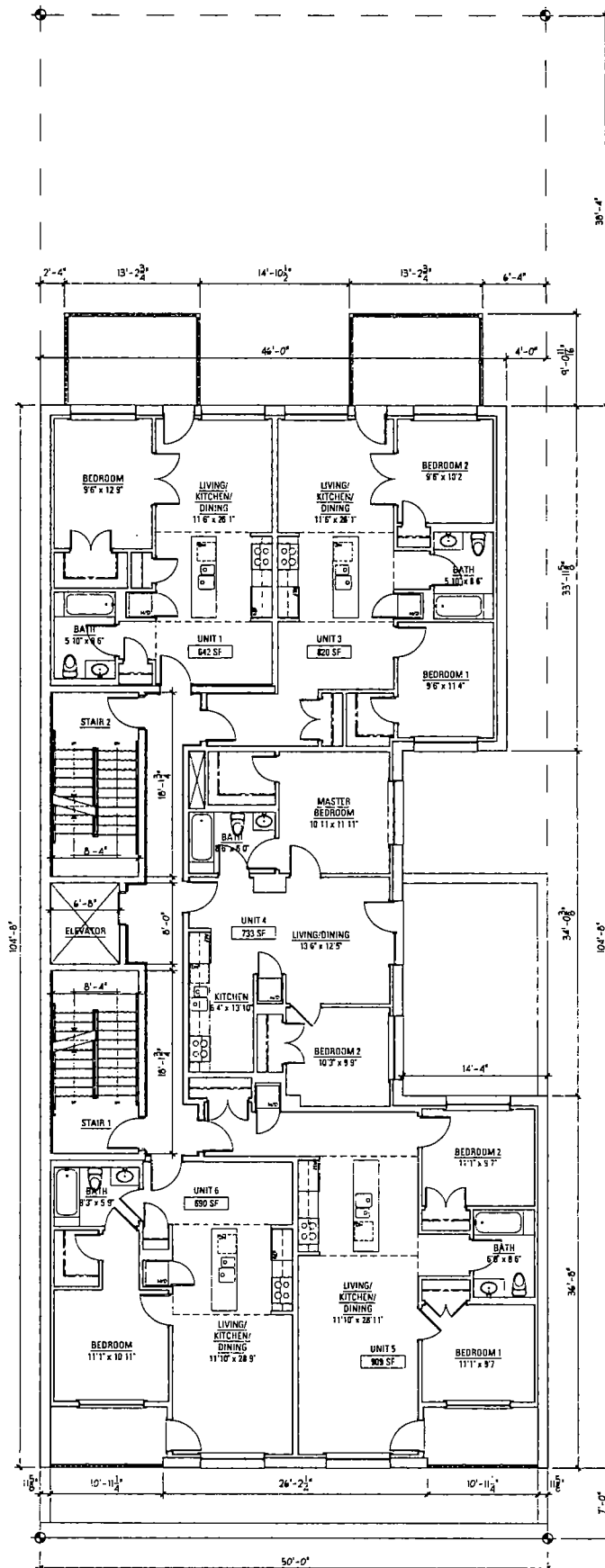
3RD - 4TH FLOOR PLAN - 4,479 SF
