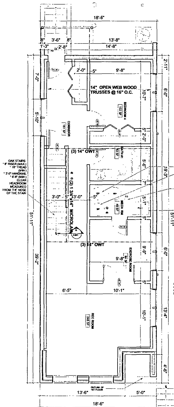
BASEMENT FLOOR 3/8" = 1'-0"
