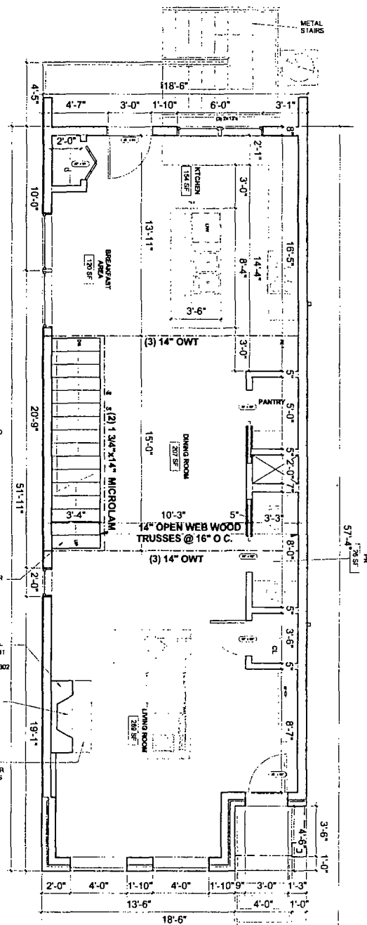
FIRST FLOOR PLAN 3/8" = 1'-0"
