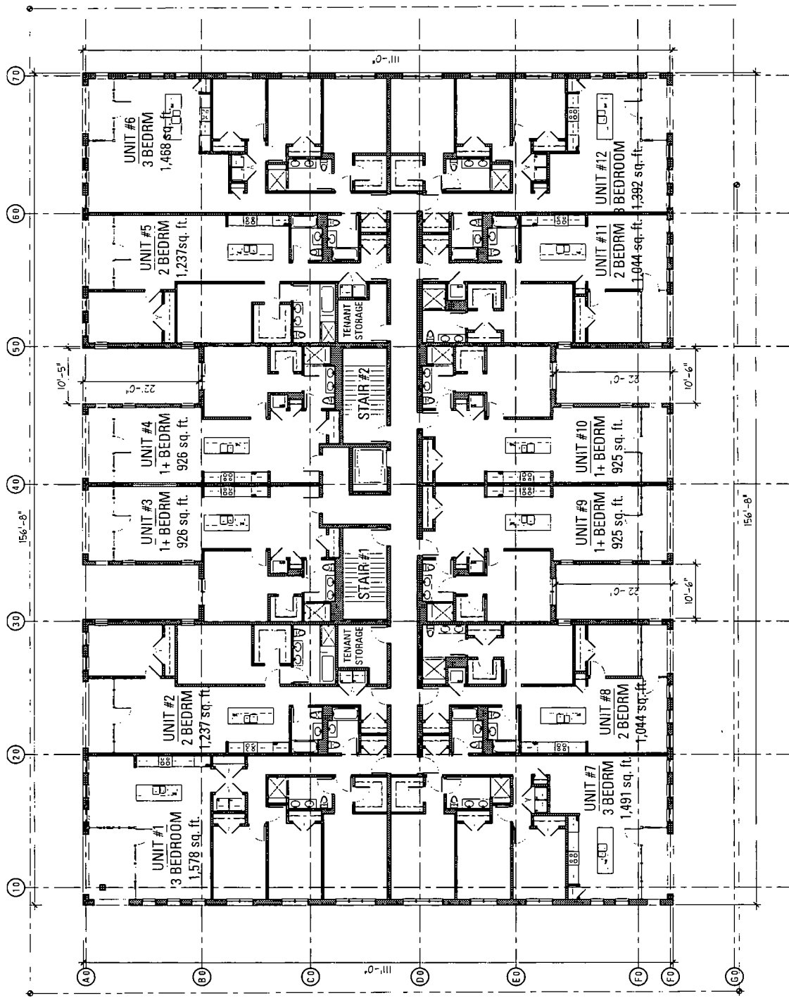
TYPICAL RESIDENTIAL FLOOR PLAN 16,485 sq. ft.
