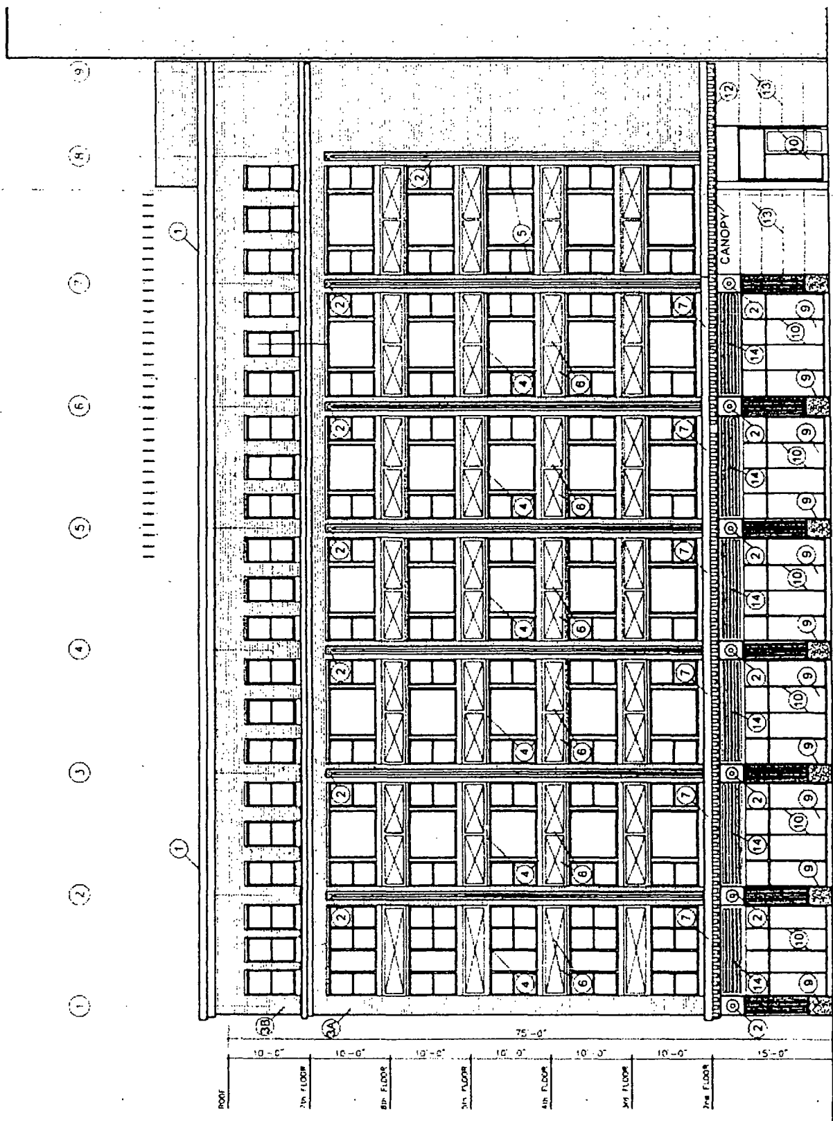
SOUTH ELEVATION
