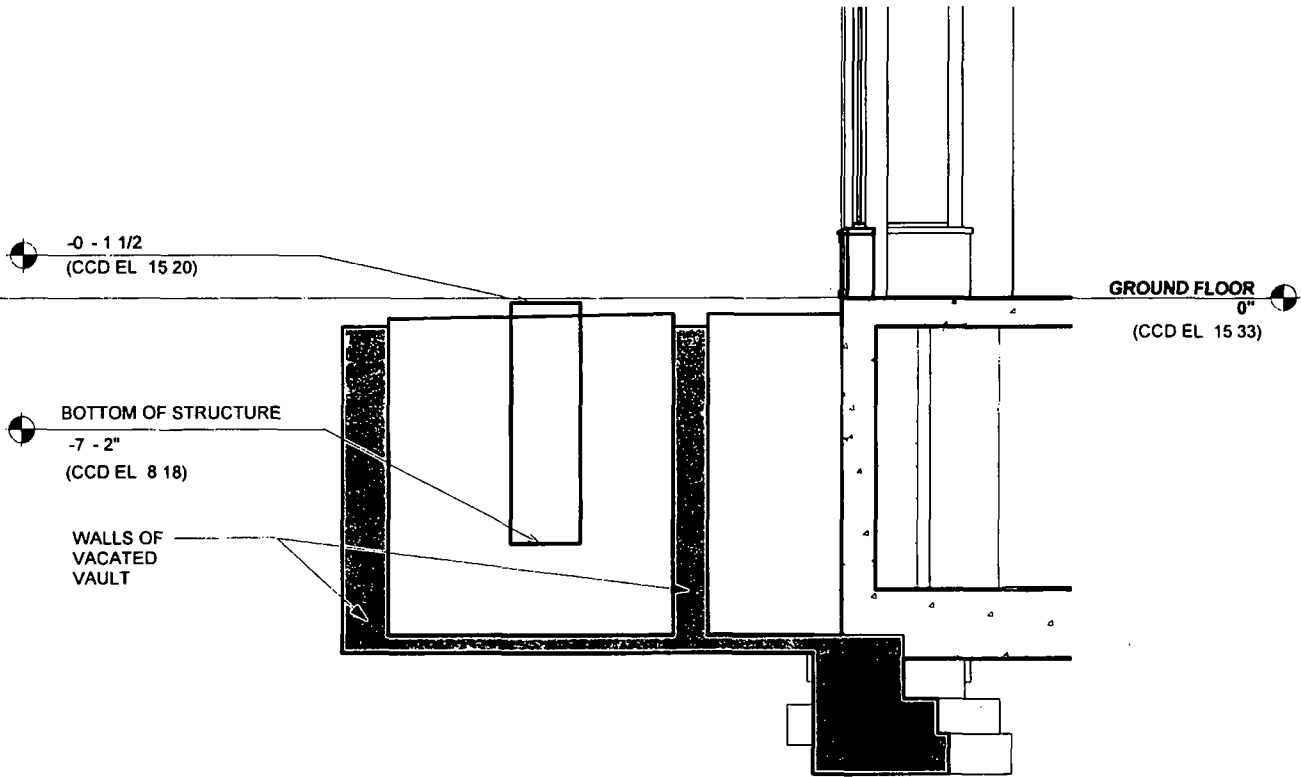
1 SECTION AT SANITARY MANHOLE PROW-4 SCALE 1/4" = 1'-0"
